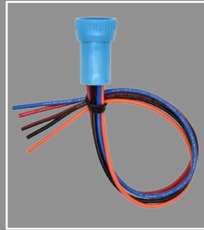
5 Wire / 2 Output Switch Harness
